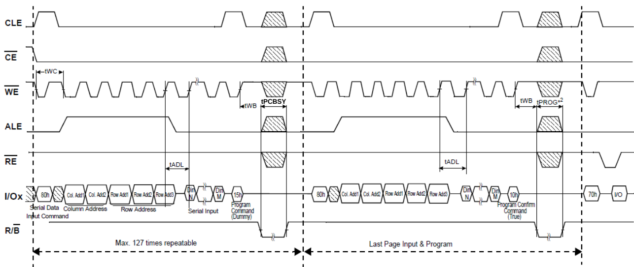
Figure 18 : cache program
